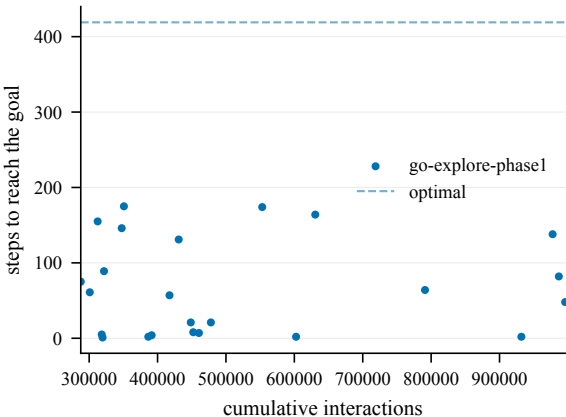
Steps to goal (train) -- EpicChase8-120@1
