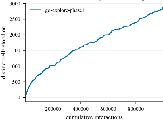
States discovered -- EpicChase8-120@1
