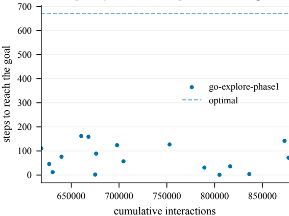
Steps to goal (train) -- EpicChase8-120@2
