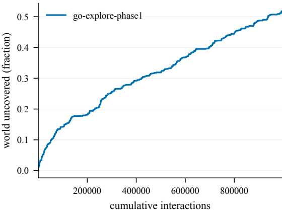
Cumulative coverage -- EpicChase8-120@3
