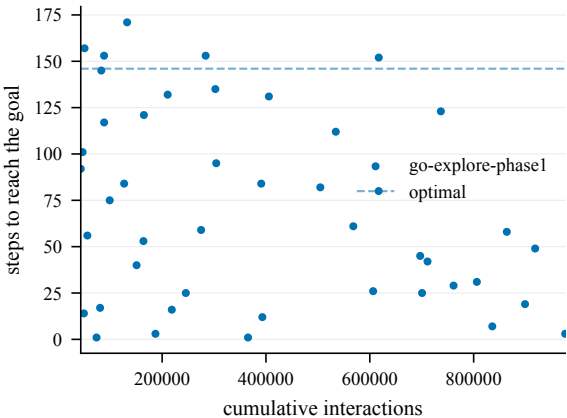
Steps to goal (train) -- EpicChase8-120@5
