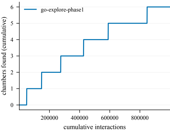
Chambers -- EpicChase8-120@6
