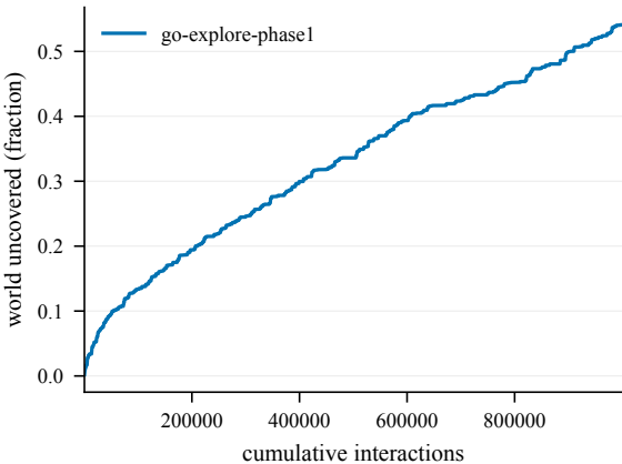
Cumulative coverage -- EpicChase8-120@6
