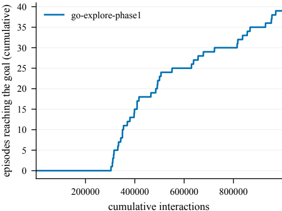
Goal reached -- EpicChase8-120@7
