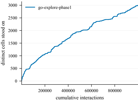
States discovered -- EpicChase8-120@8
