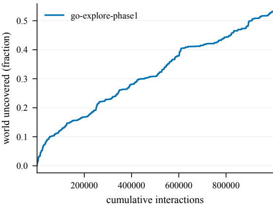
Cumulative coverage -- EpicChase8-120@9
