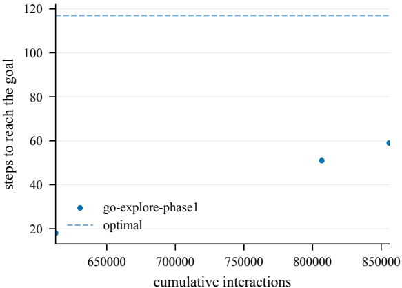
Steps to goal (train) -- EnlargedChamberCount10-180@5
