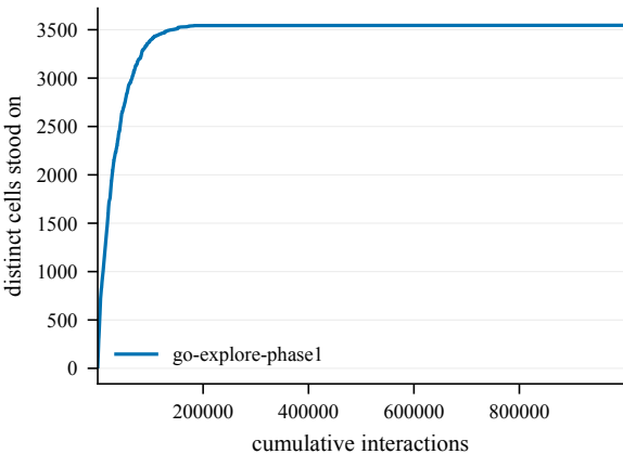
States discovered -- EnlargedChamberCount2-60
