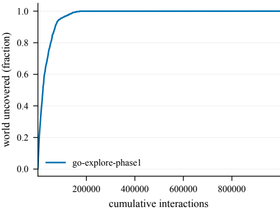
Cumulative coverage -- EnlargedChamberCount2-60@1
