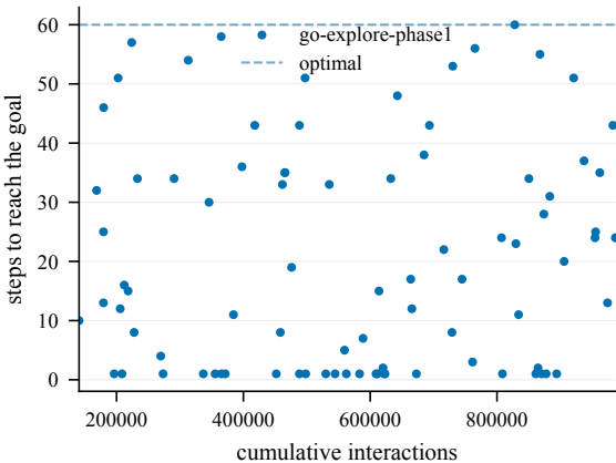
Steps to goal (train) -- EnlargedChamberCount2-60@1
