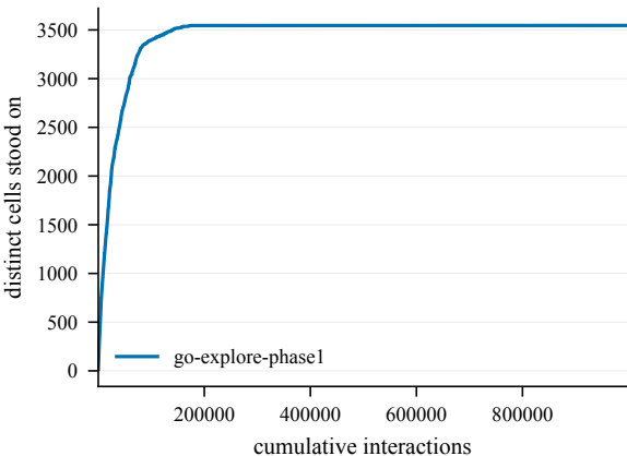
States discovered -- EnlargedChamberCount2-60@1
