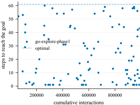
Steps to goal (train) -- EnlargedChamberCount2-60@2
