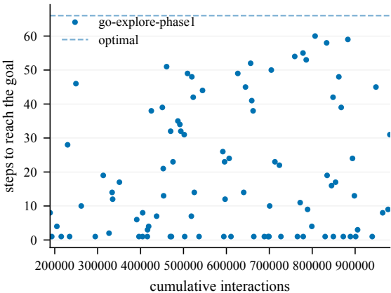
Steps to goal (train) -- EnlargedChamberCount2-60@4
