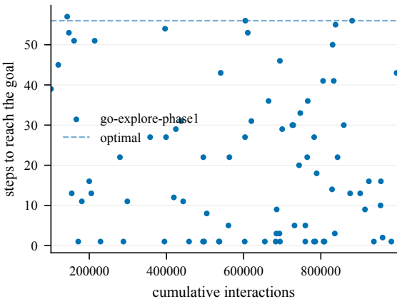
Steps to goal (train) -- EnlargedChamberCount2-60@5
