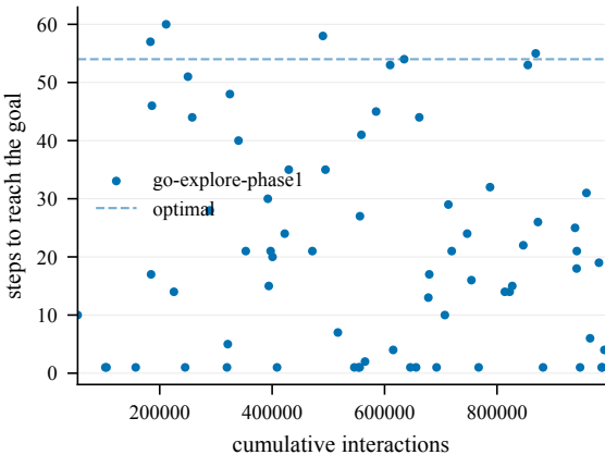
Steps to goal (train) -- EnlargedChamberCount2-60@6
