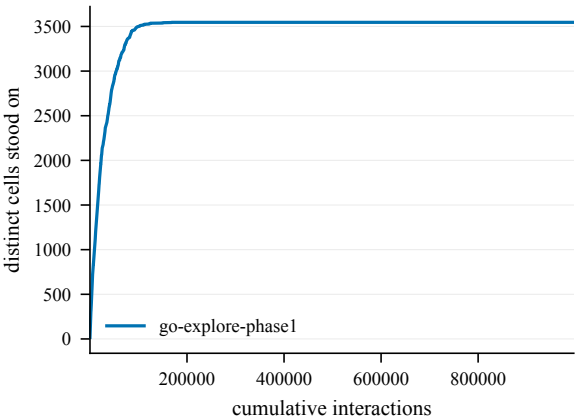
States discovered -- EnlargedChamberCount2-60@9
