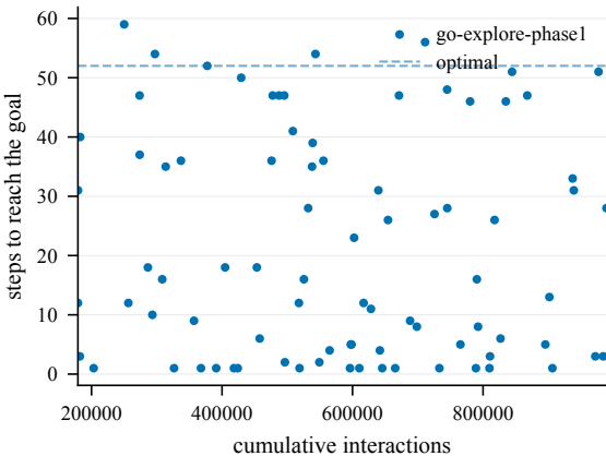
Steps to goal (train) -- EnlargedChamberCount3-60@3
