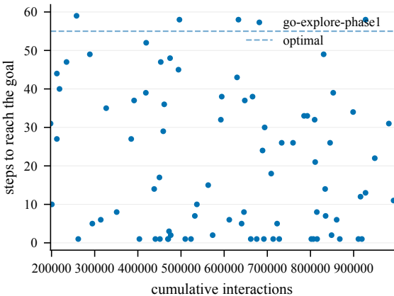
Steps to goal (train) -- EnlargedChamberCount3-60@5
