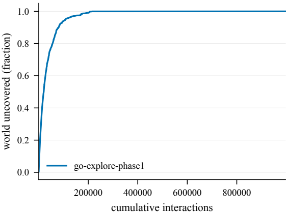
Cumulative coverage -- EnlargedChamberCount3-60@7
