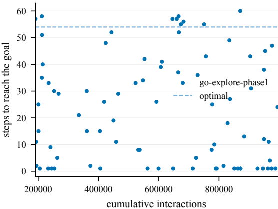
Steps to goal (train) -- EnlargedChamberCount3-60@9
