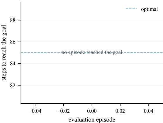
Steps to goal (eval) -- EnlargedChamberCount4-80
