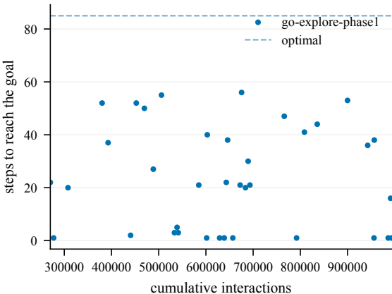
Steps to goal (train) -- EnlargedChamberCount4-80
