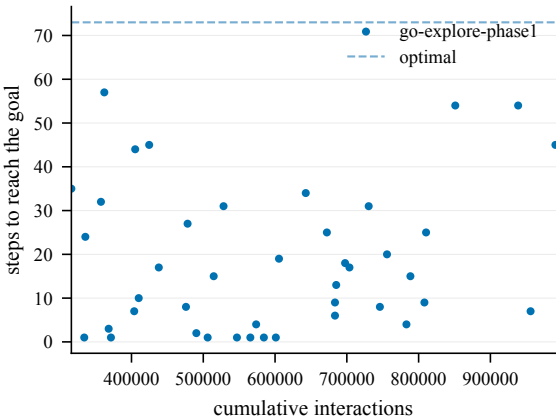
Steps to goal (train) -- EnlargedChamberCount4-80@3
