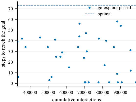
Steps to goal (train) -- EnlargedChamberCount4-80@4
