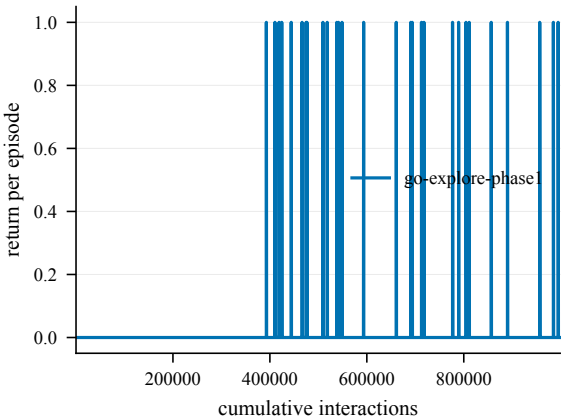
Return -- EnlargedChamberCount4-80@5
