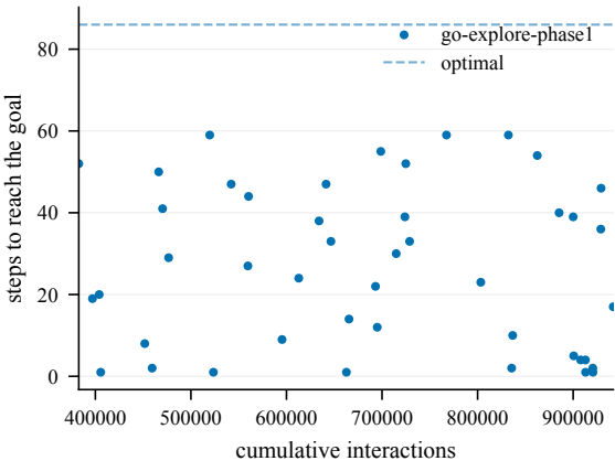
Steps to goal (train) -- EnlargedChamberCount4-80@7
