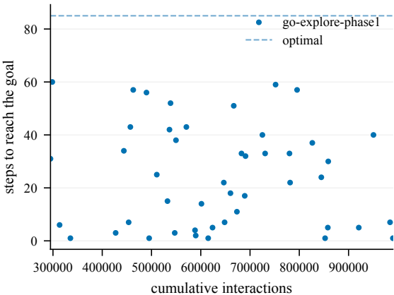
Steps to goal (train) -- EnlargedChamberCount4-80@8
