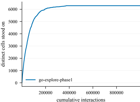
States discovered -- EnlargedChamberCount4-80@8
