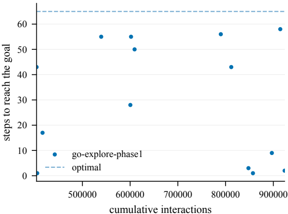
Steps to goal (train) -- EnlargedChamberCount5-100@2
