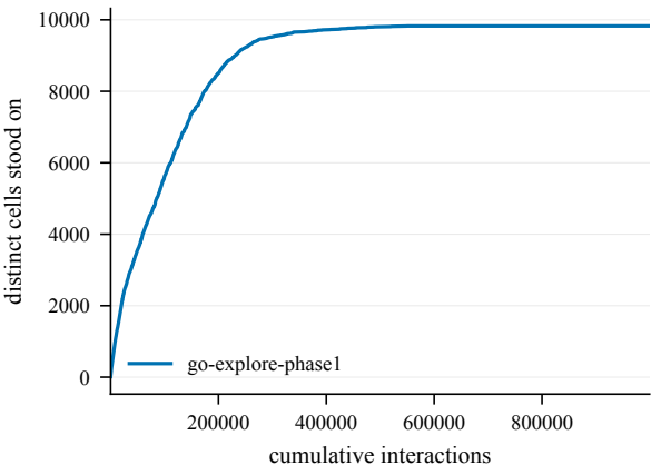
States discovered -- EnlargedChamberCount5-100@2
