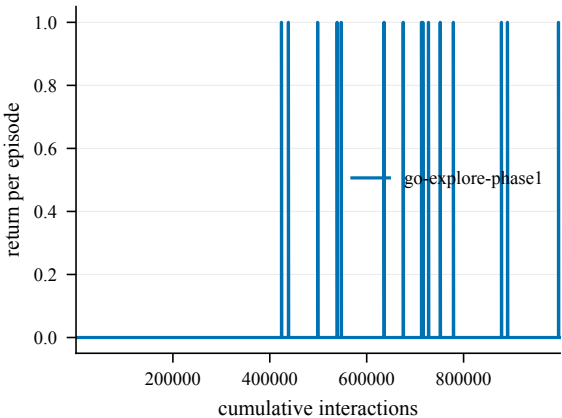
Return -- EnlargedChamberCount5-100@5
