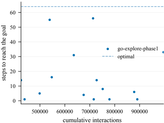
Steps to goal (train) -- EnlargedChamberCount5-100@5
