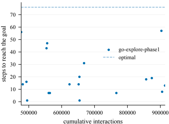
Steps to goal (train) -- EnlargedChamberCount5-100@8
