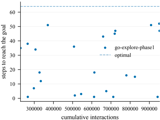
Steps to goal (train) -- EnlargedChamberCount5-100@9
