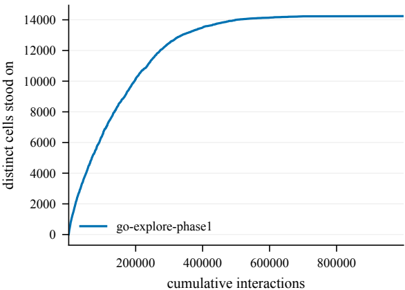
States discovered -- EnlargedChamberCount6-120
