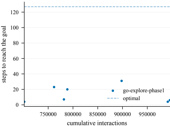
Steps to goal (train) -- EnlargedChamberCount6-120@5
