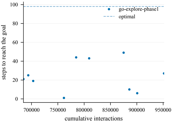
Steps to goal (train) -- EnlargedChamberCount6-120@7
