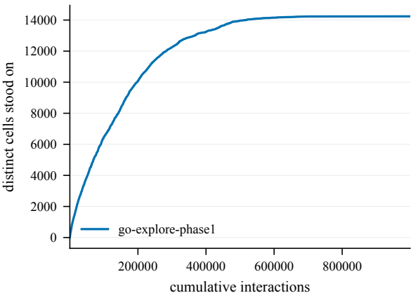
States discovered -- EnlargedChamberCount6-120@8
