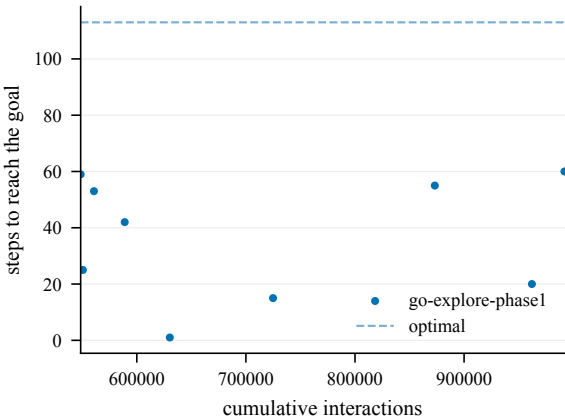
Steps to goal (train) -- EnlargedChamberCount6-120@9
