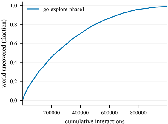
Cumulative coverage -- EnlargedChamberCount8-150@3
