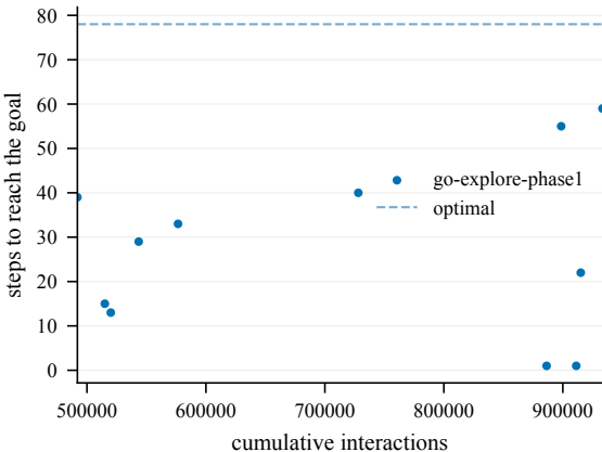
Steps to goal (train) -- EnlargedChamberCount8-150@4
