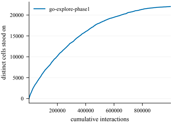
States discovered -- EnlargedChamberCount8-150@4
