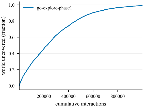
Cumulative coverage -- EnlargedChamberCount8-150@7
