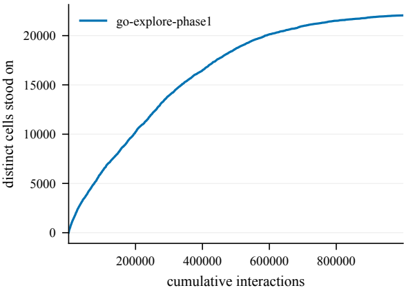
States discovered -- EnlargedChamberCount8-150@7
