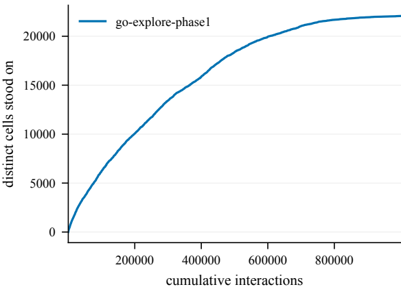
States discovered -- EnlargedChamberCount8-150@8
