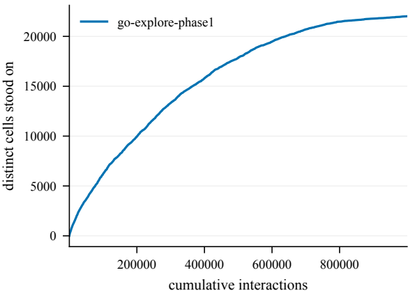
States discovered -- EnlargedChamberCount8-150@9
